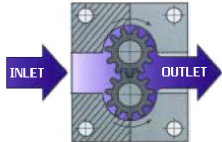
Precision Gear Metering
