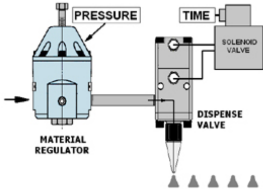
Time and Pressure Metering
