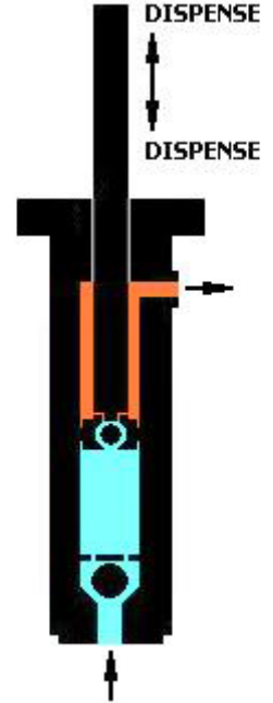
Double Acting Piston
