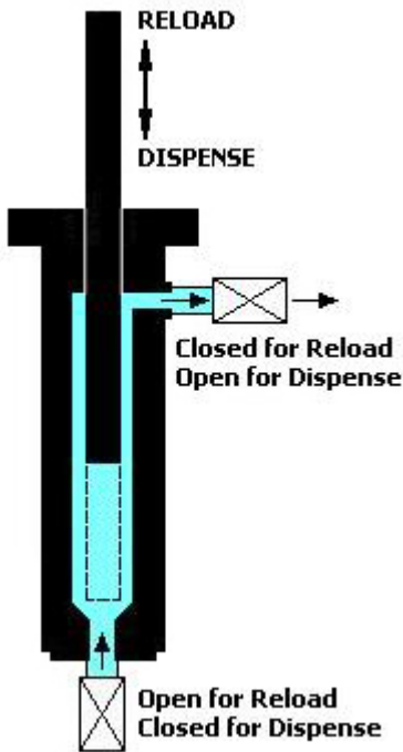
Positive Rod Displacement
